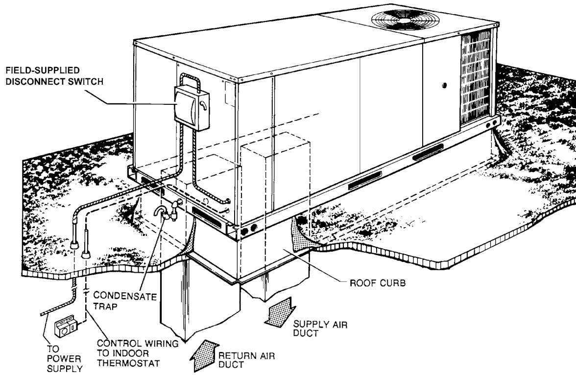
FIGURE 8 - TYPICAL APPLICATIONS
